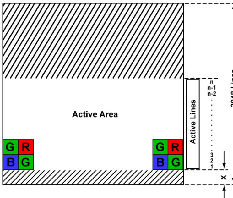
FIGURE 48. Bayer 2
